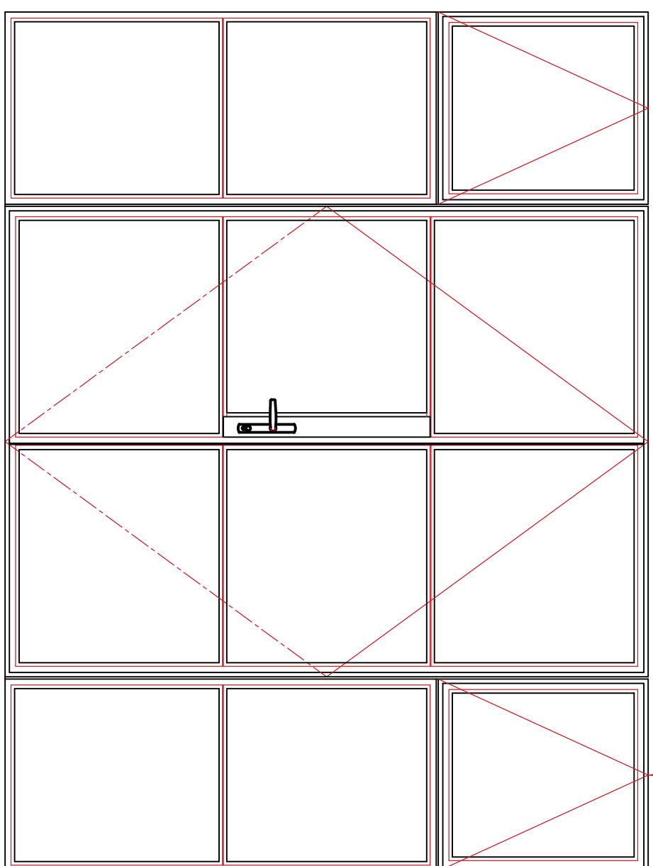
TYPICAL DOUBLE DOOR WITH SIDE-LIGHT AND VENTILATORS
