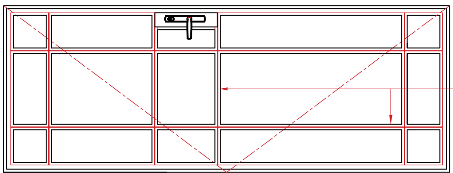
TYPICAL SINGLE DOOR
