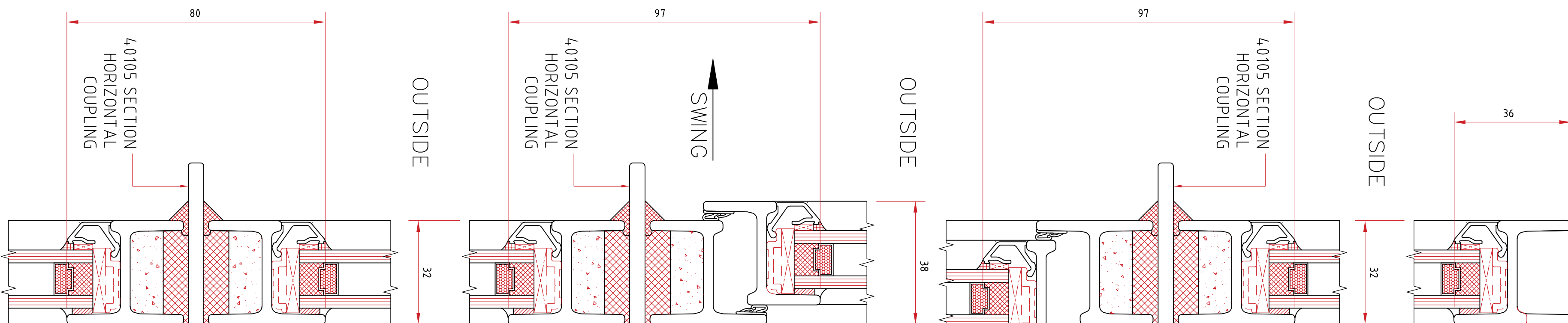
TYPICAL DOUBLE DOOR WITH TOP-LIGHT AND SIDE-LIGHTS
