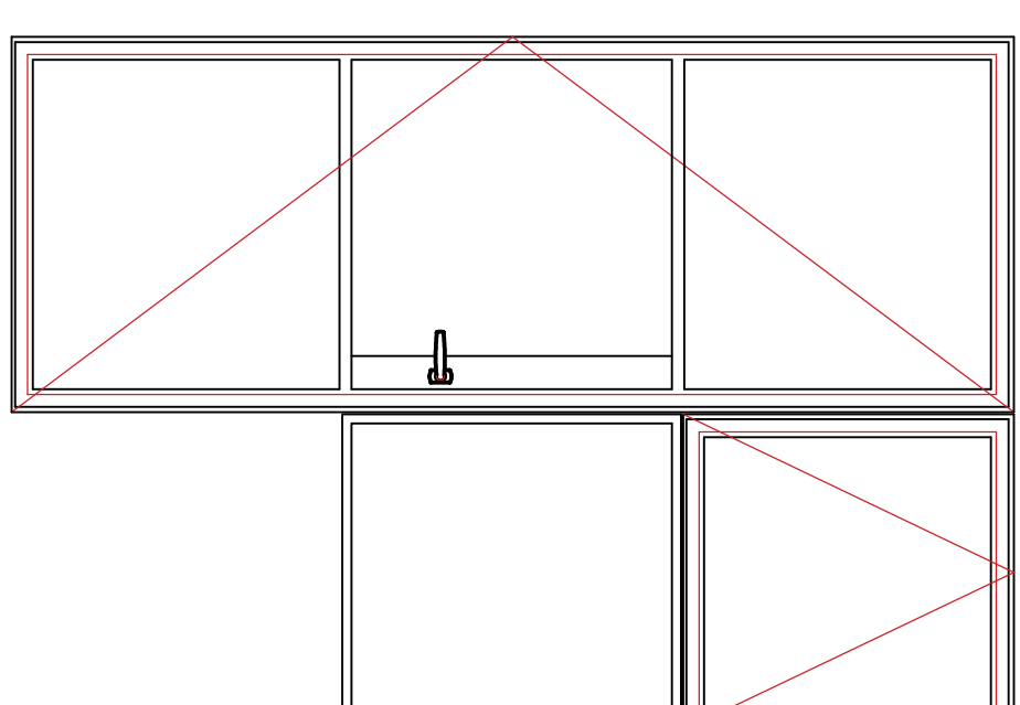
SINGLE DOOR & SIDELIGHTS-COUPLED ASSEMBLY, EXAMPLE
