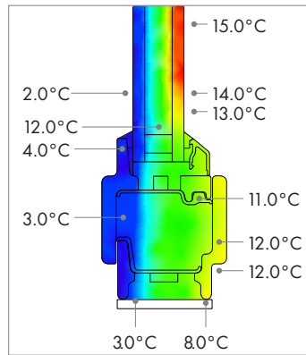
Thermal gradients produced using Dartwin Frame Simulator PRO software to ISO 10077-2:2017
